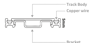
Ultra-thin Track Channel
